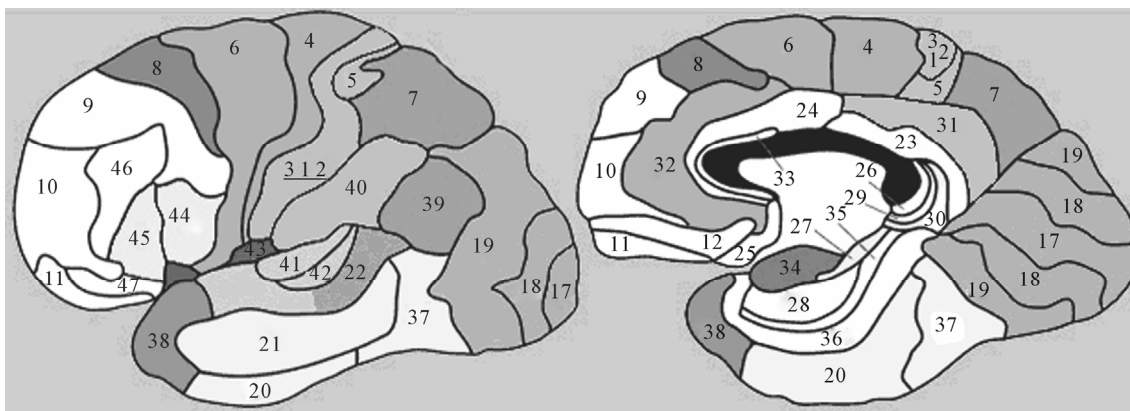
Figure 2. Map illustrating the Brodmann's areas (BA).
